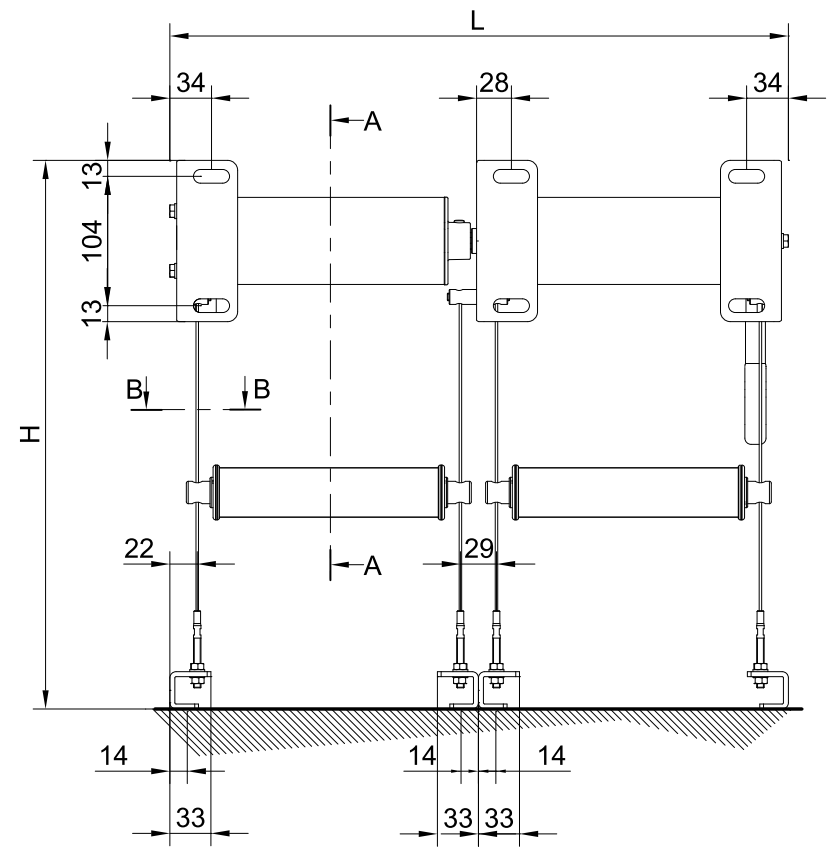
vista posteriore rear view
